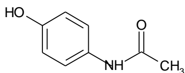
paracetamol MW 151.17
