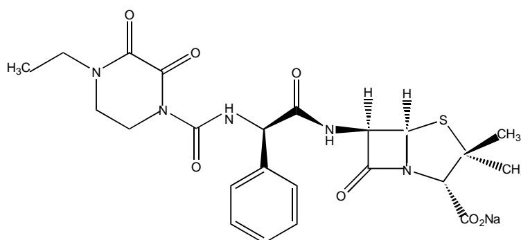
Piperacillin sodium
