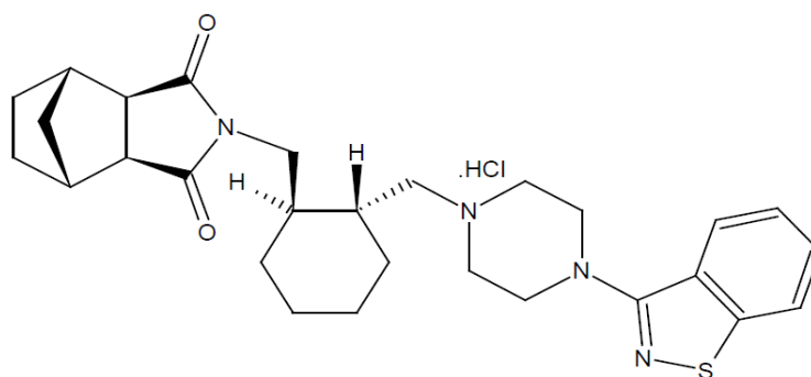
Figure 1. Chemical structure of Lurasidone hydrochloride
